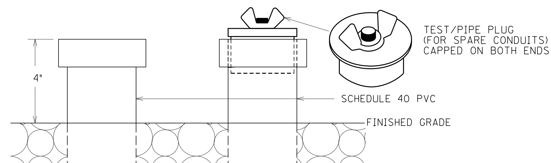
TEST/PIPE PLUG (FOR SPARE CONDUITS) DETAIL
