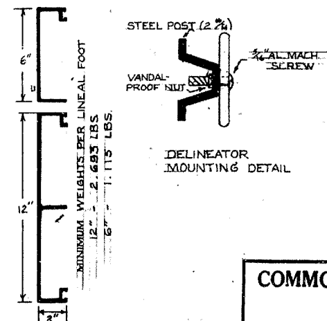
TYPICAL SECTIONS ALUMINUM SIGN PANEL EXTRUSIONS
