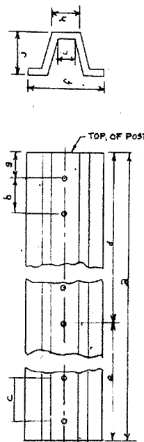
TYPICAL DIMENSIONS FOR STEEL POSTS
