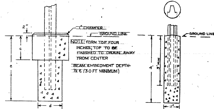
MOUNTING DETAILS
