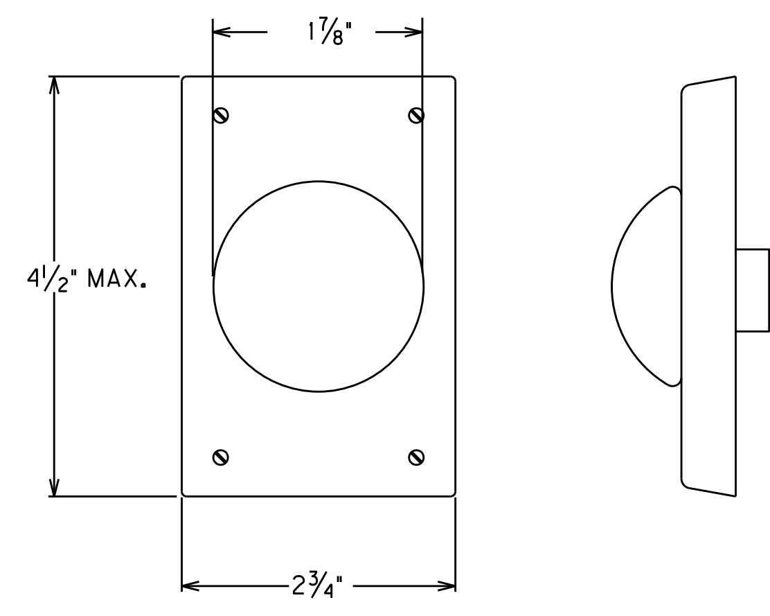
PED DETECTOR
