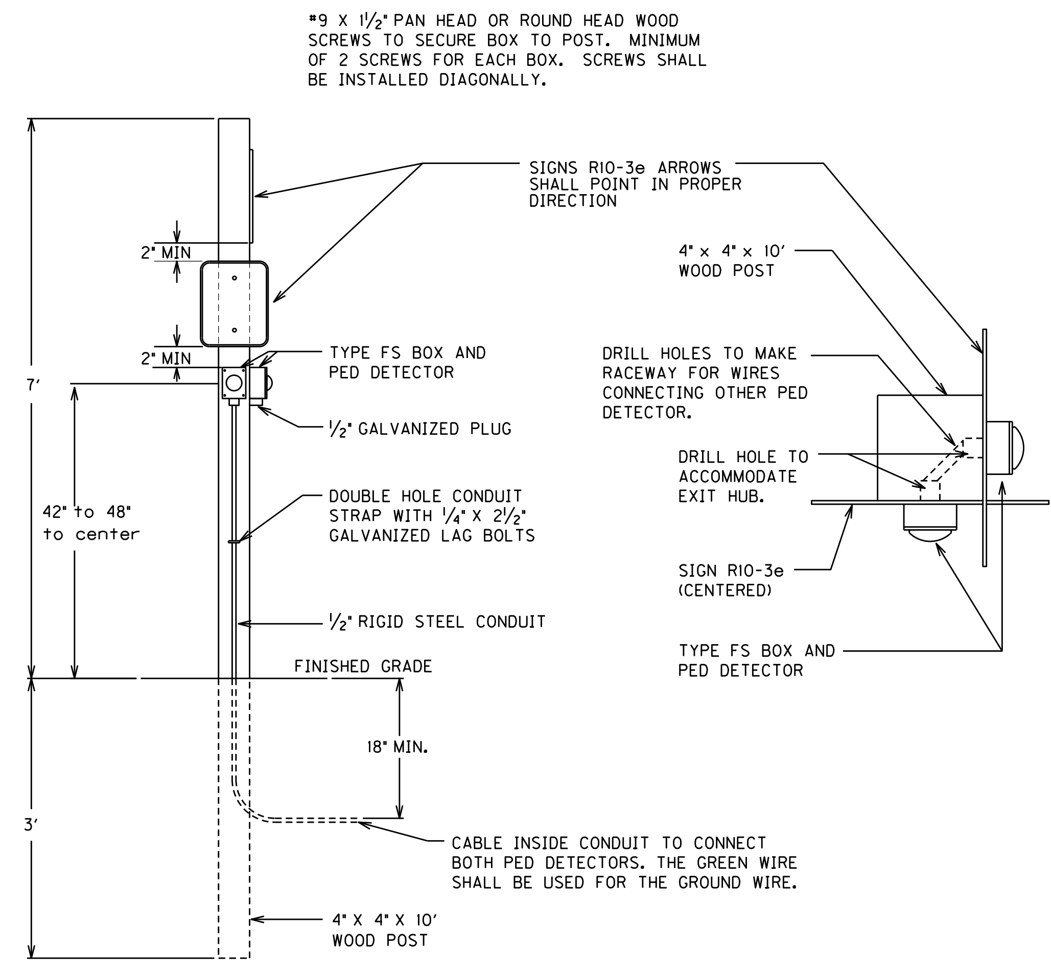
PED DETECTOR ON WOOD POST DETAIL
