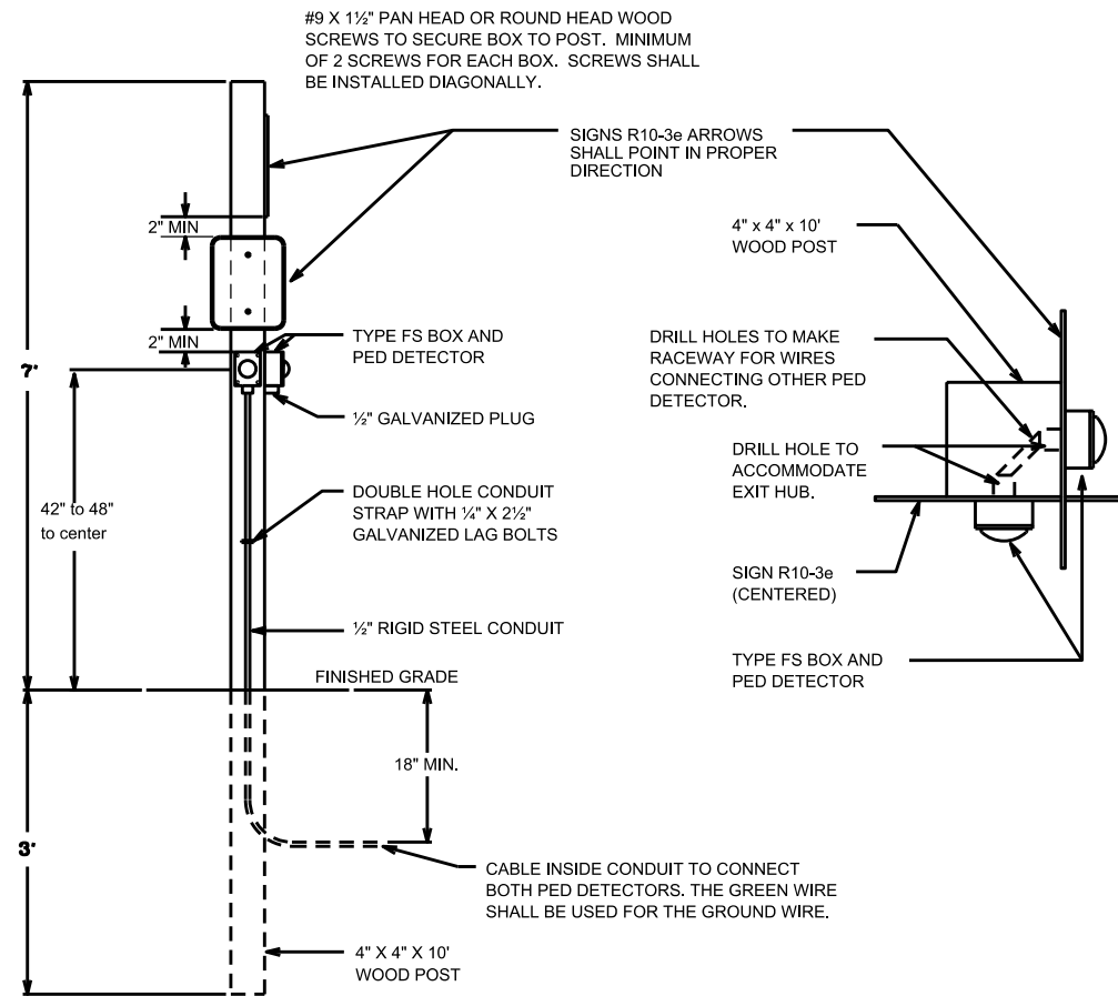
PED DETECTOR ON WOOD POST DETAIL
