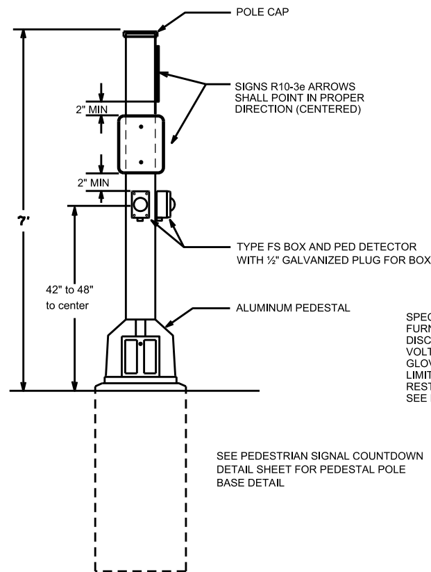
PEDESTAL POST DETAIL FOR PED DETECTORS & SIGNS
