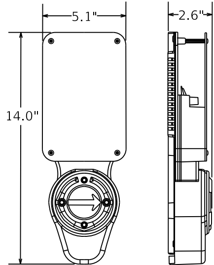
AUDIBLE PED DETECTOR
