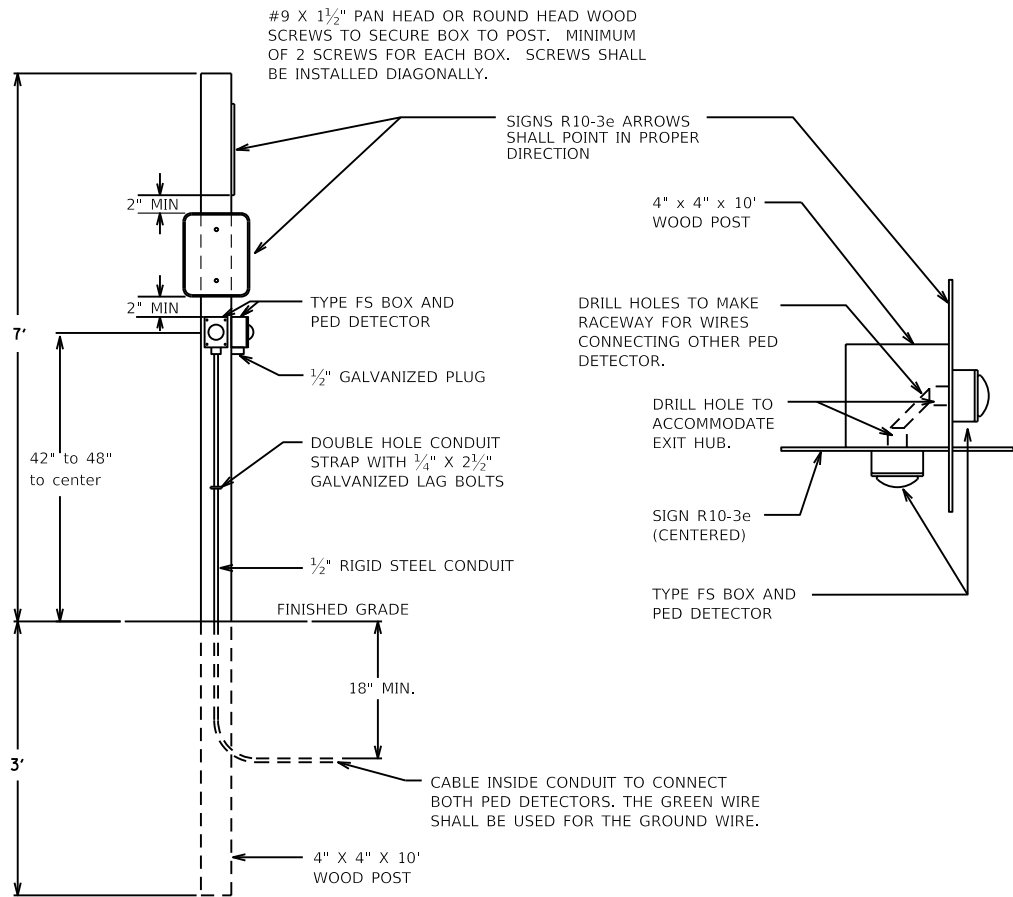
PED DETECTOR ON WOOD POST DETAIL
